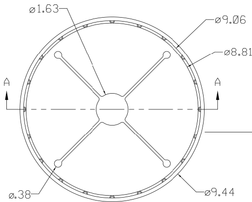
VB STABILIZER 5 1/4 PLASTIC VALVE BOX BOTTOM 101/106 BELL
