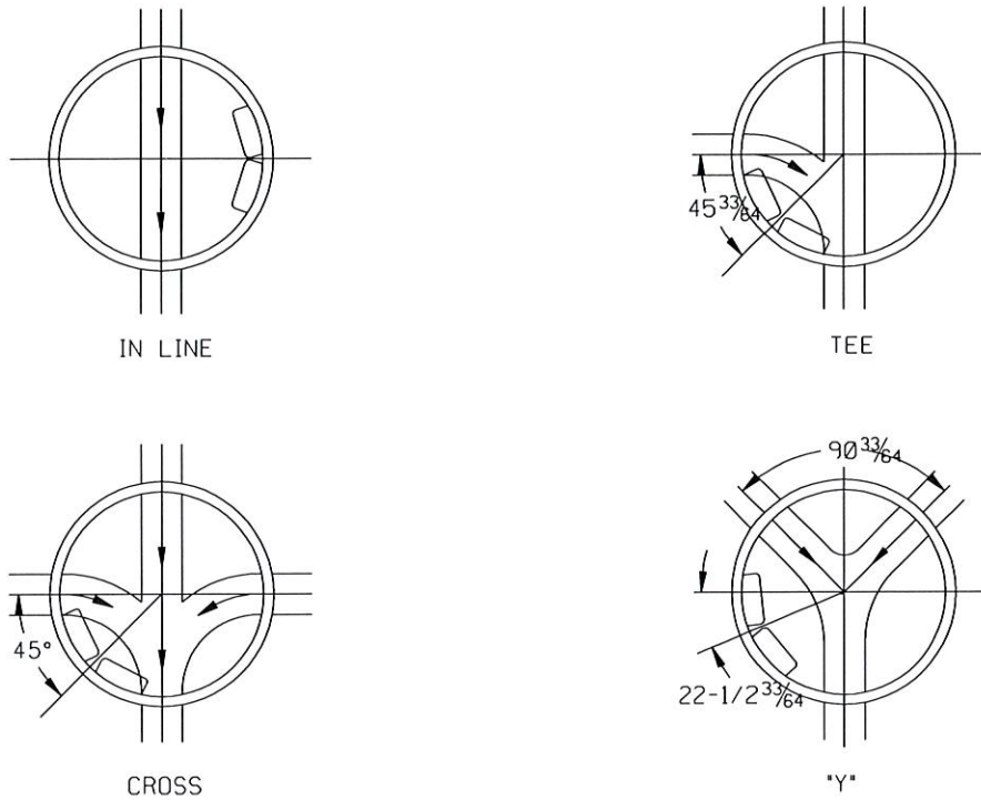
LOCATION OF MANHOLE STEPS
