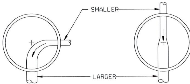
TYPICAL MANHOLE INVERT DETAILS
