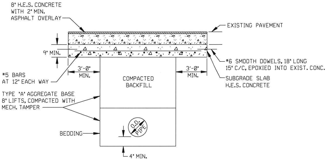
TYPICAL SECTION: ASPHALT PAVEMENT
