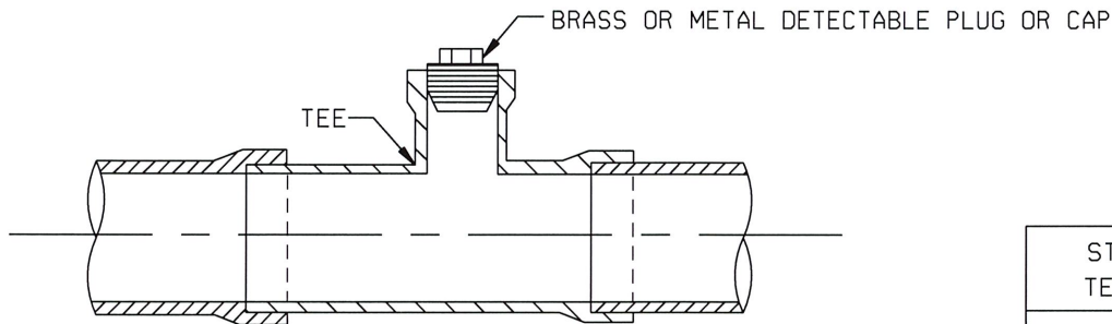
TYPICAL CROSS-SECTION
