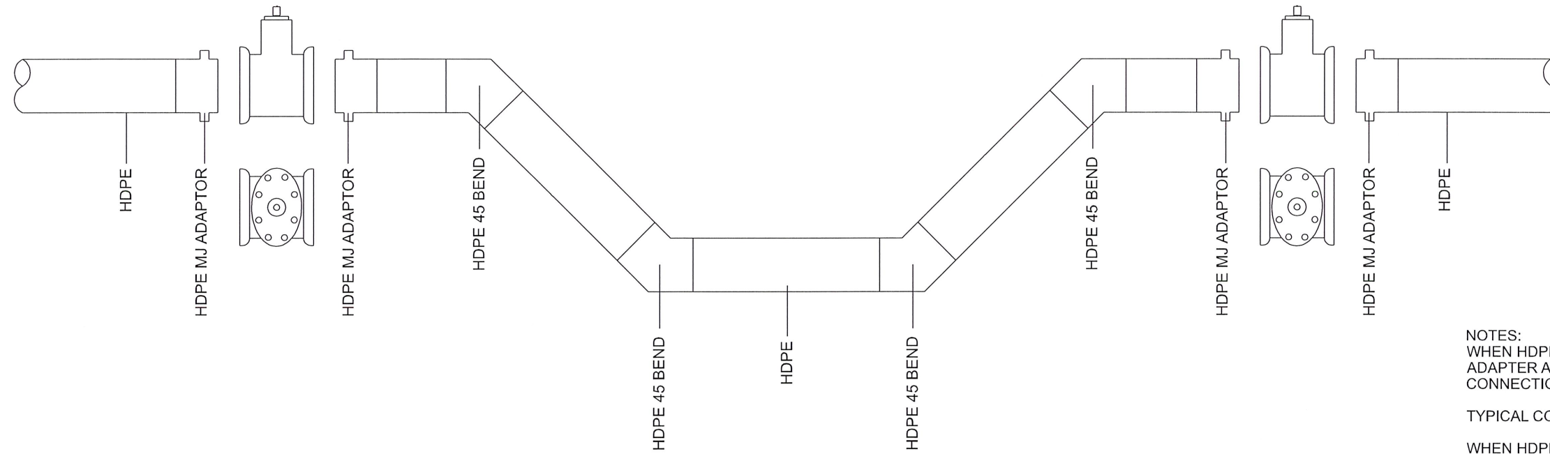
HDPE HORIZONTAL / VERTICAL REALIGNMENT USING FITTINGS
